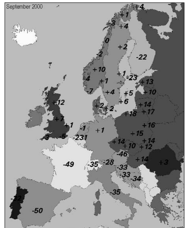
Figure 30: Differences between EVRF2000 zero level and the zero levels of national height systems in Europe (in cm).
