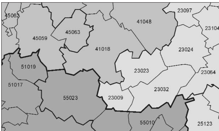
Figure 14: Administrative boundaries in a cross border area.
