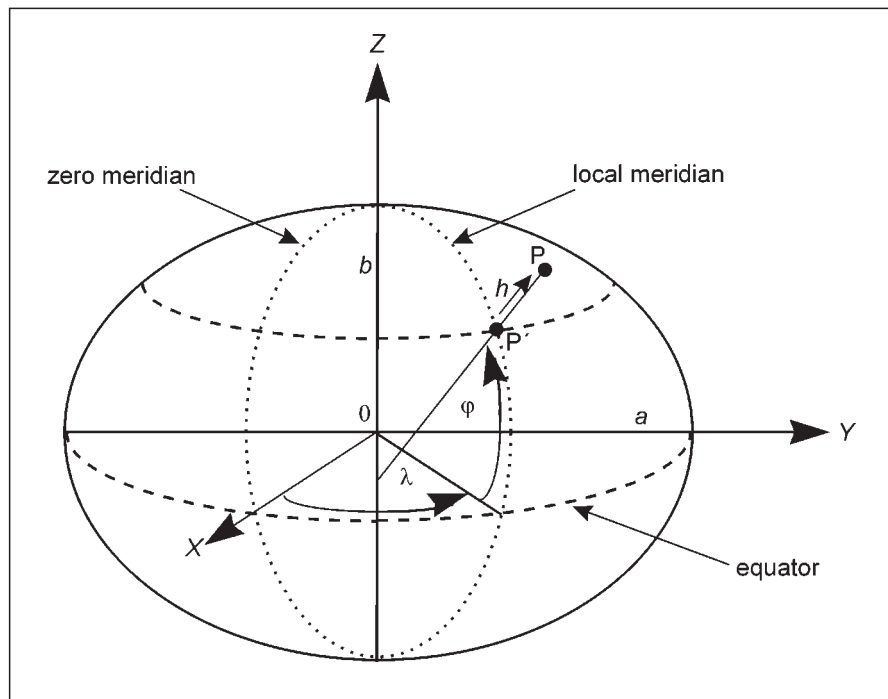
Figure 32: Cartesian coordinates and ellipsoidal coordinates.
