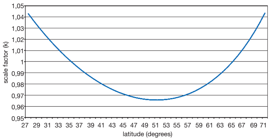
Figure 33: Variation of the scale factor ( k ) against latitude.
