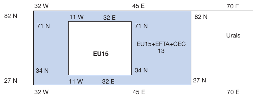
Figure 1: the area of interest.
