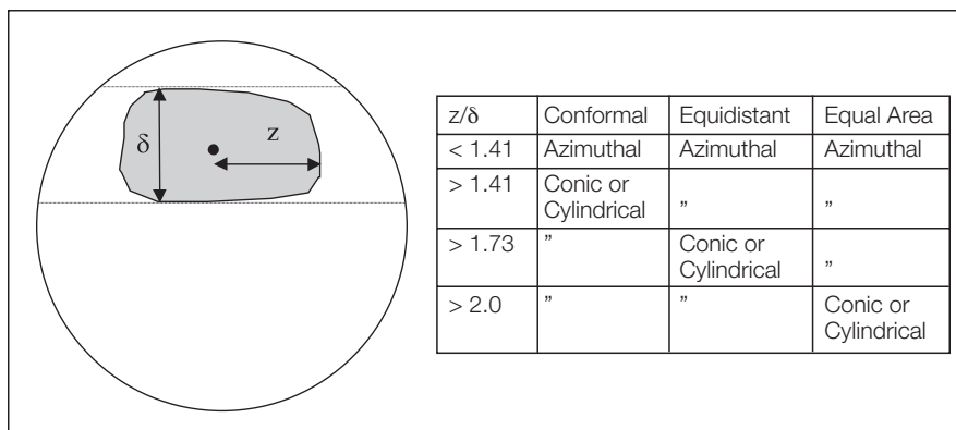
Figure 7: Young's Rule.
