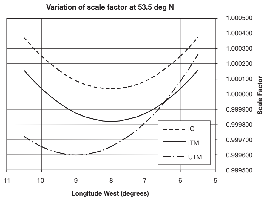
Figure 13: Variation of scale factor at 53° 30' N.
