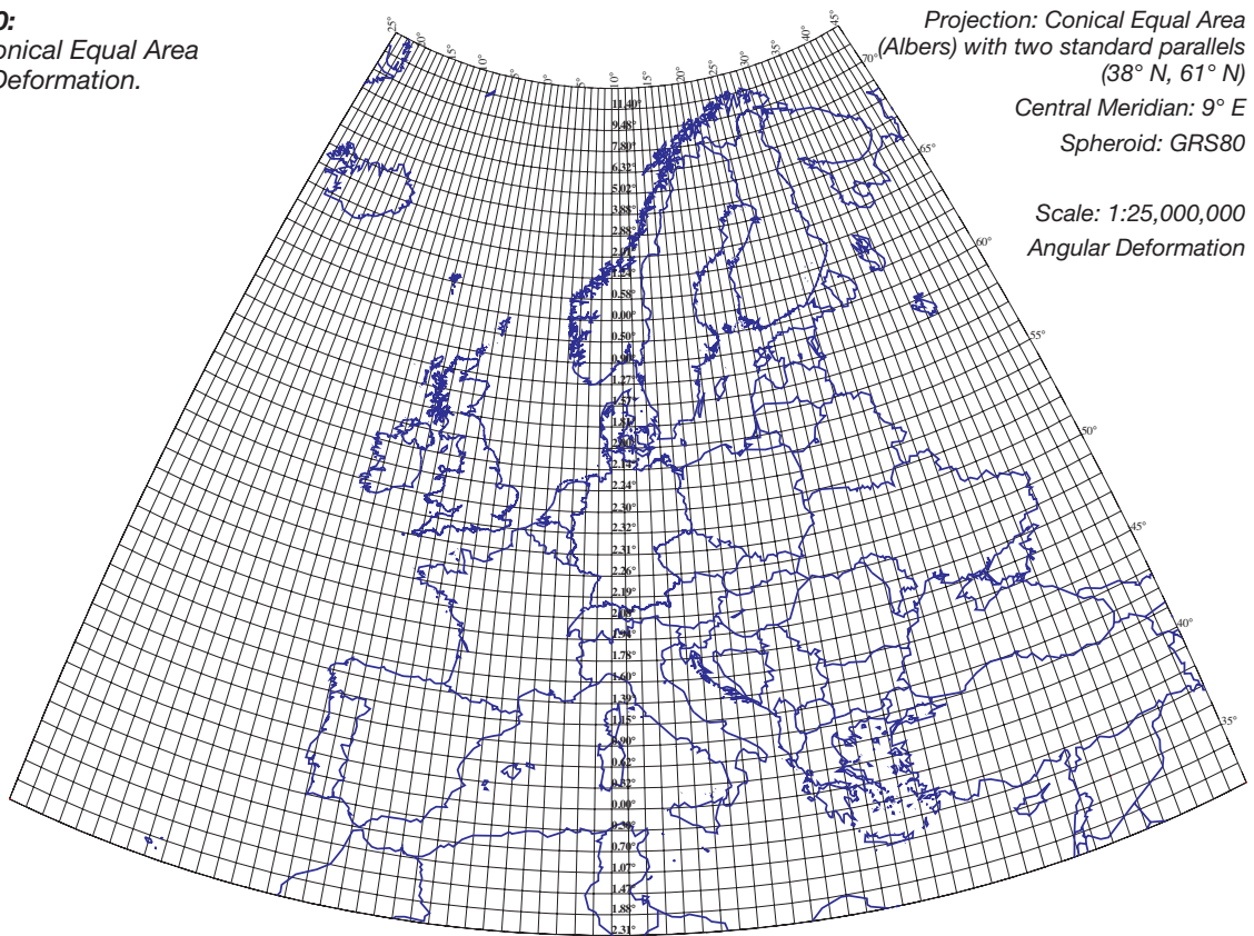
Figure 11: Alberd Conical Equal Area Scale error.
