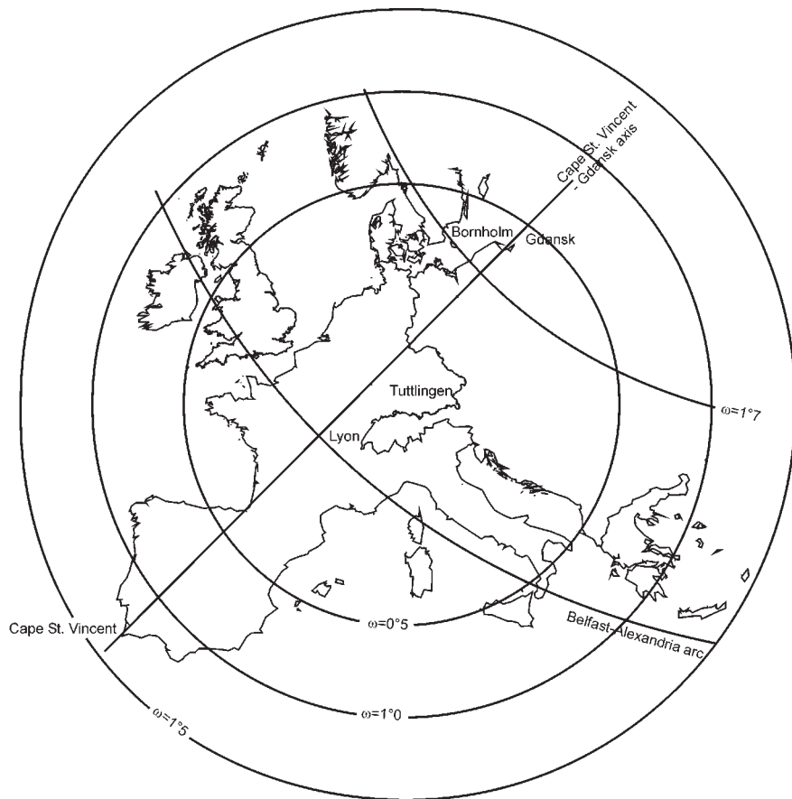
Figure 23: Maling's deformation comparison of an oblique equal area conical projection with an oblique equal area azimuthal projection (from Maling p. 261).
