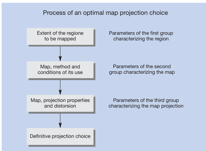
Figure 21: Workflow of a projection choice after Bugayevskiy.
