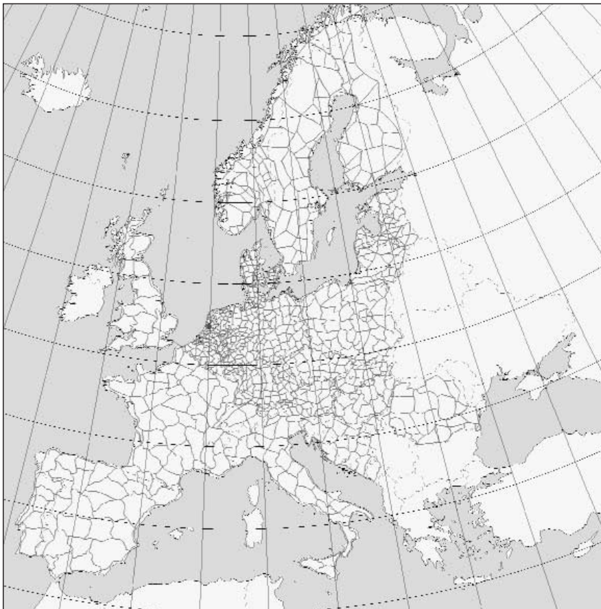
Figure 26: United European Levelling Network 1995 (UELN-95/98 – extended for Estonia, Latvia, Lithuania and Romania).
