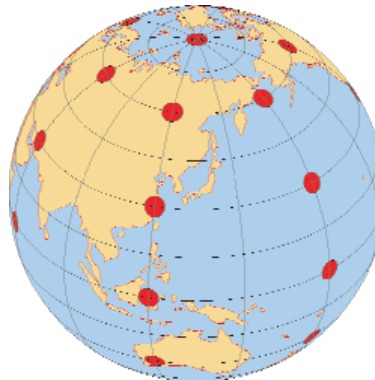
Figure 20: Orthographic projection in an oblique aspect with Tissot's indicatrices.
