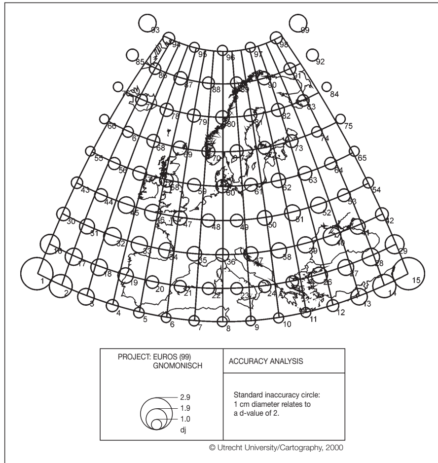
Figure 16: Accuracy analysis Gnomonic projection for Europe
