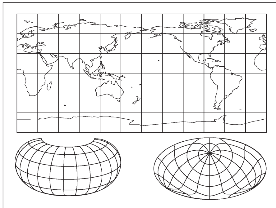
Figure 19: Curvature of the graticule lines.
